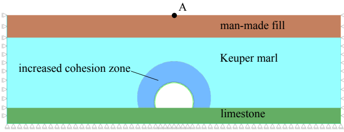
Figure 1: Ground layers considered in the model.
