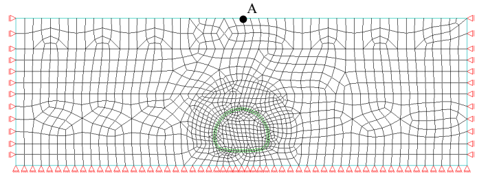
Figure 2: Finite element mesh.
