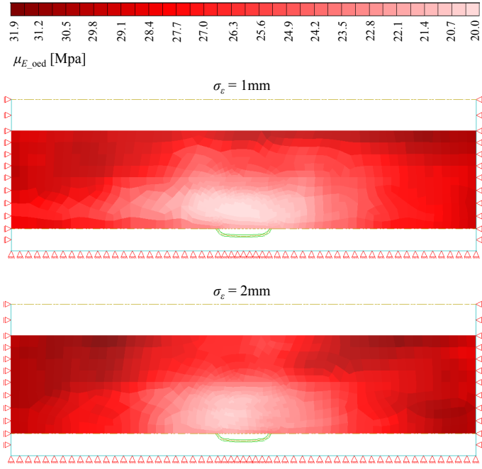
Figure 4: Posterior mean of the oedometric stiffness modulus E_{\text{oeed}} of the Keuper marl layer.
